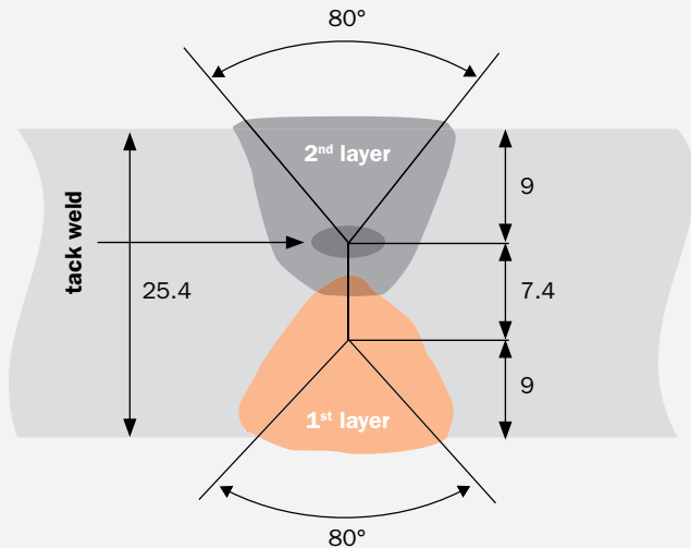
FMI process parameters for a sheet thickness of 25.4 mm (1").
